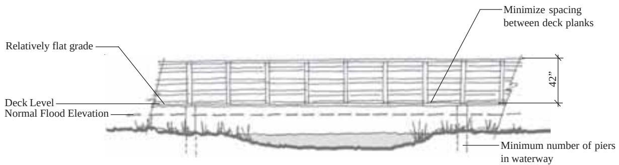
Figure 20 Wetland Boardwalk
